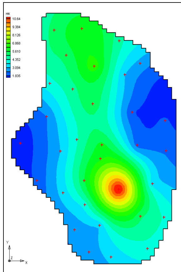
Figure 14-1 Pilot Points and Resulting Conductivity Field
