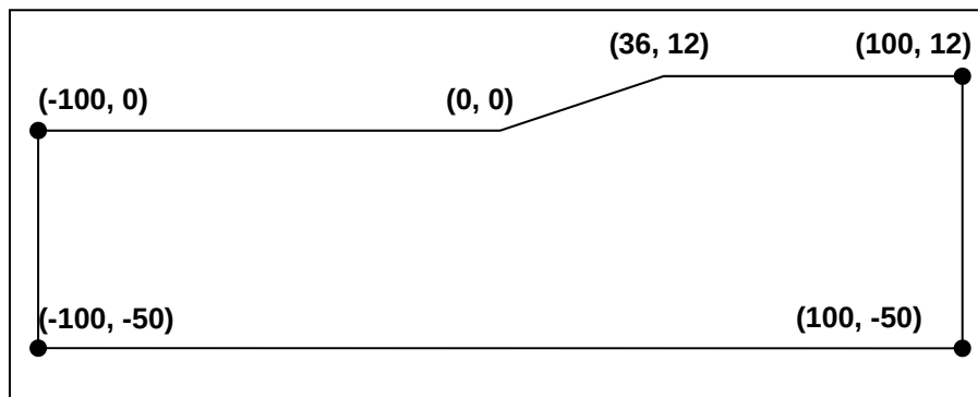
Figure 12. Embankment coordinates.
